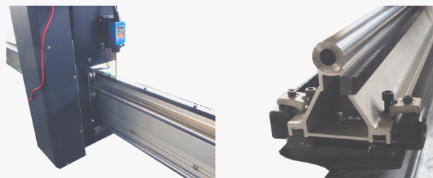
INDEPENDENT INTEGRATED SHAPE OF ALUMINUM DIE
